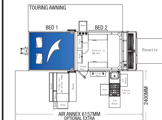
Floor Plan
