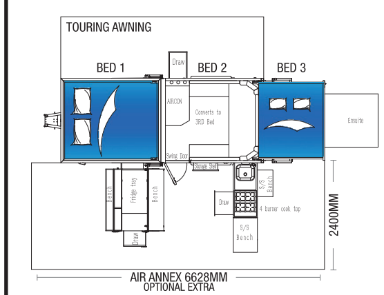
Floor Plan
